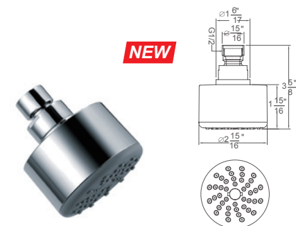
SH0150100 (Chrome) SH0150400 (Brushed Nickel) Multifunction showerhead
