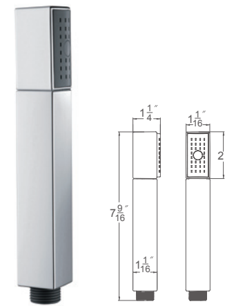
HSLD10102 (Chrome) HSLD10402 (Brushed Nickel) Handshower with flexible hose
