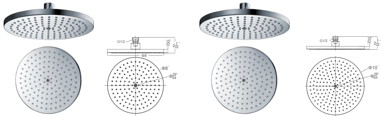
RSS240100-8 (Chrome) RSS240400-8 (Brushed Nickel) 8" Round Rain Showerhead with Air Mixture
