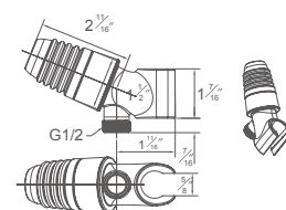
HH2200100 (Chrome) HH2200400 (Brushed Nickel) Adjustable Wall Mount Bracket
