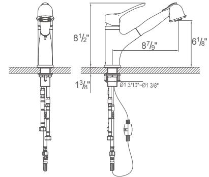
AB50 3712 Single-Lever Pull-Out Spray Sink Faucet AB50 3712BN Brushed Nickel AB50 3712C Chrome
