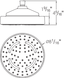
SHM230101 (Chrome) SHM230401 (Brushed Nickel) Showerhead
