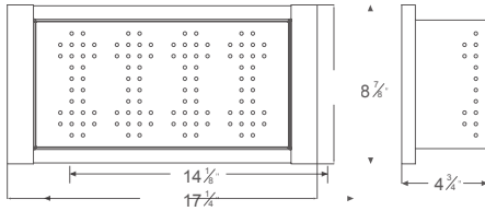
COL120 Colander Material: 304 Stainless Steel Finish: Polished Satin
