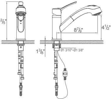
AB50 3711 Single-Lever Pull-Out Spray Sink Faucet AB50 3711BN Brushed Nickel AB50 3711C Chrome
