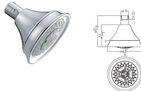
SH0170100 (Chrome) SH0170400 (Brushed Nickel) Multifunction Showerhead
