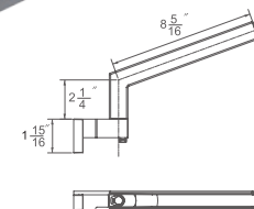
MN03 (Chrome) MN04 (Brushed Nickel) Wall Mount Bracket and Arm for HSLD10102
