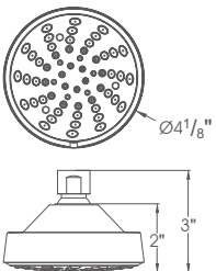
SH0160100 (Chrome) SH0160400 (Brushed Nickel) Showerhead
