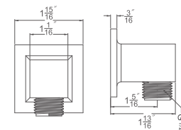
WCA050100 (Chrome) WCA050400 (Brushed Nickel) Shower wall-mount supply elbow
