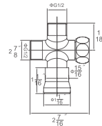
DTR090100 (Chrome) DTR090400 (Brushed Nickel) Push Pull Shower Diverter
