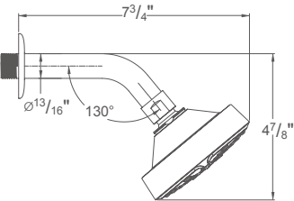
SH0160101 (Chrome) SH0160401 (Brushed Nickel) Showerhead with arm and flange
