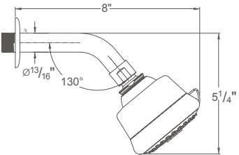
SHM090101 (Chrome) SHM090401 (Brushed Nickel) Showerhead with arm and flange
