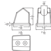
HH0400100 (Chrome) HH0400400 (Brushed Nickel) Shower wall bracket (fixed)
