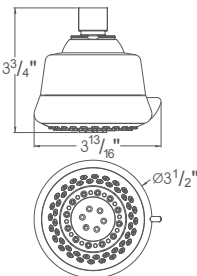
SHM090100 (Chrome) SHM090400 (Brushed Nickel) Showerhead
