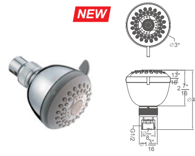
SH0080100 (Chrome) SH0080400 (Brushed Nickel) Multifunction Showerhead
