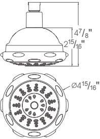
SH0200100 (Chrome) SH0200400 (Brushed Nickel) Showerhead
