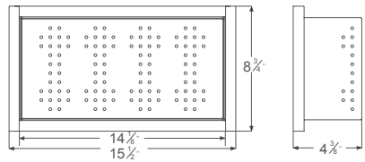
COL118 Colander Material: 304 Stainless Steel Finish: Polished Satin
