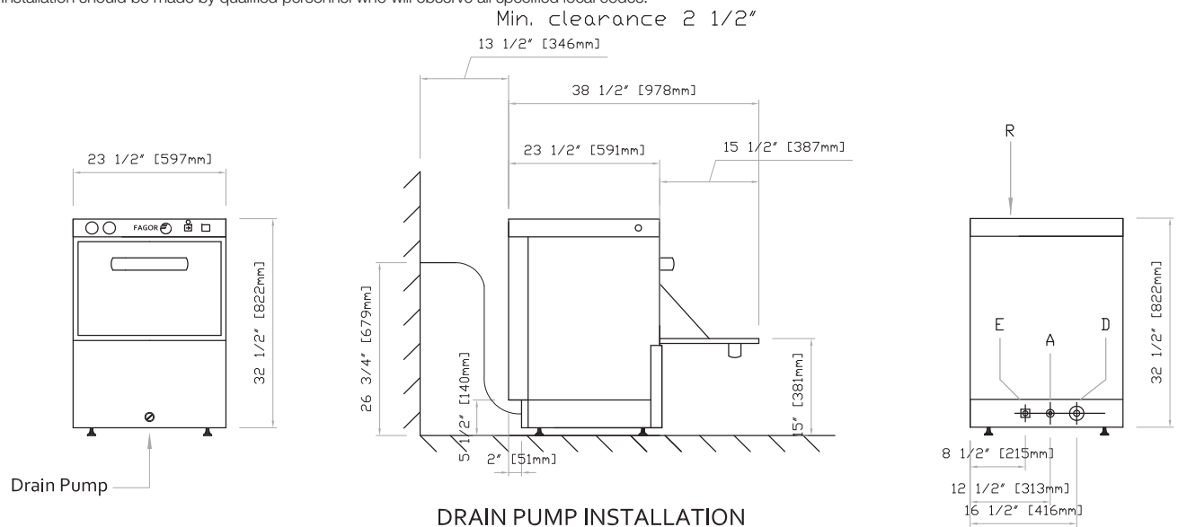
Front View
