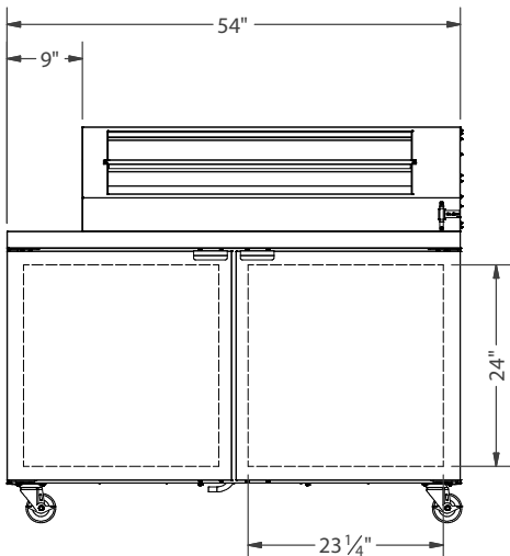
FRONT ZR152 ZF152
